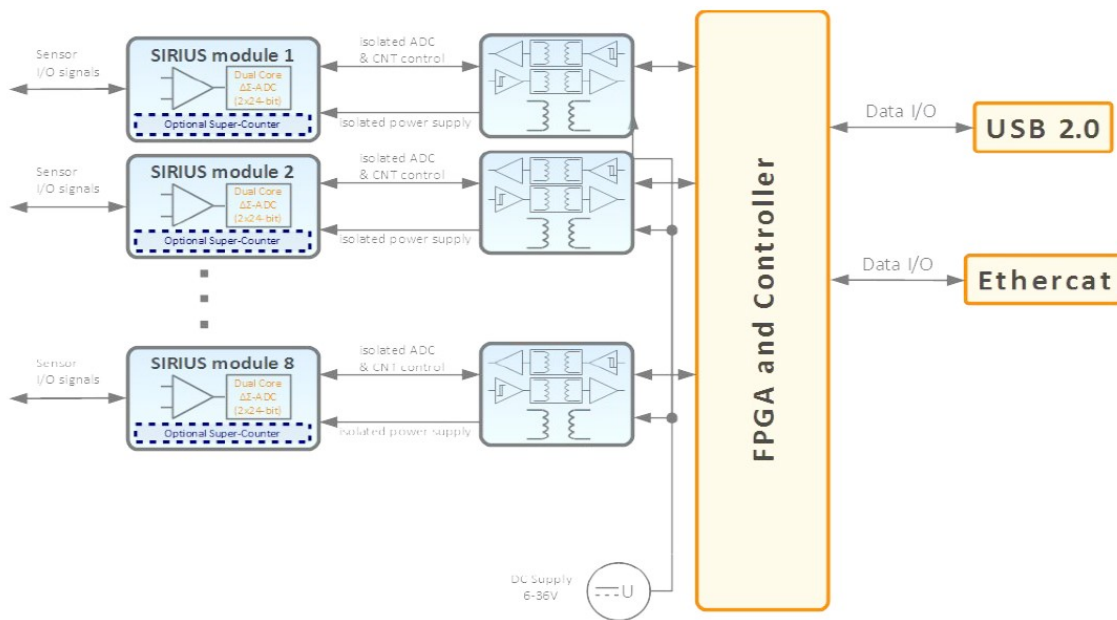
EtherCAT® Motherboard
