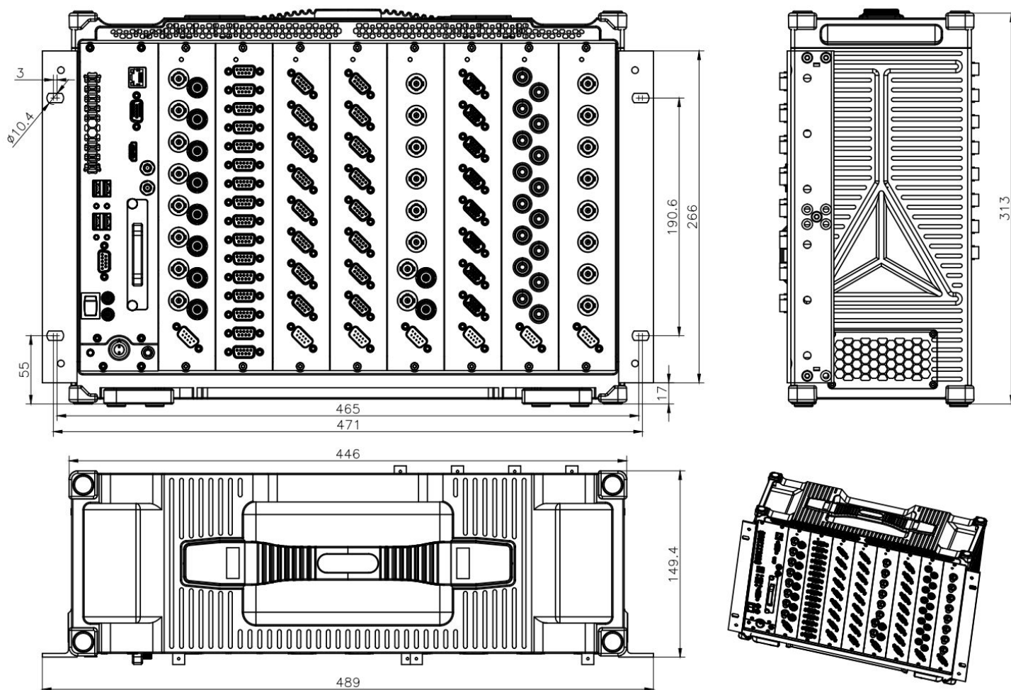
Dimensions: SIRIUS-R8
