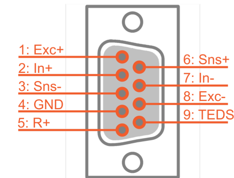
HS-STG connector: pin-out (DSUB-9 female)
