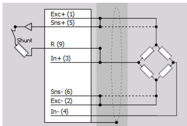
Full bridge
