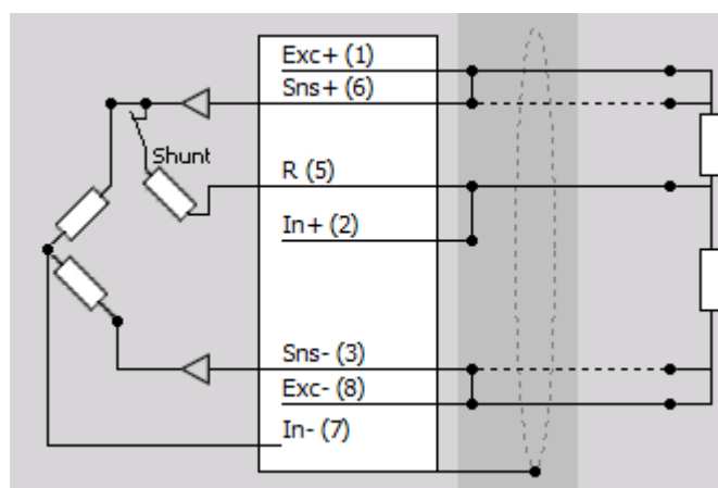
Half bridge
