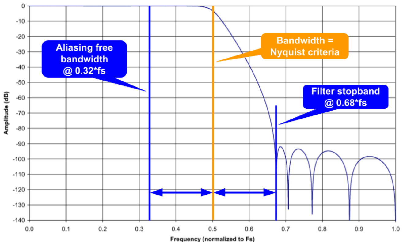
Bandwidth vs. Aliasing-free bandwidth
