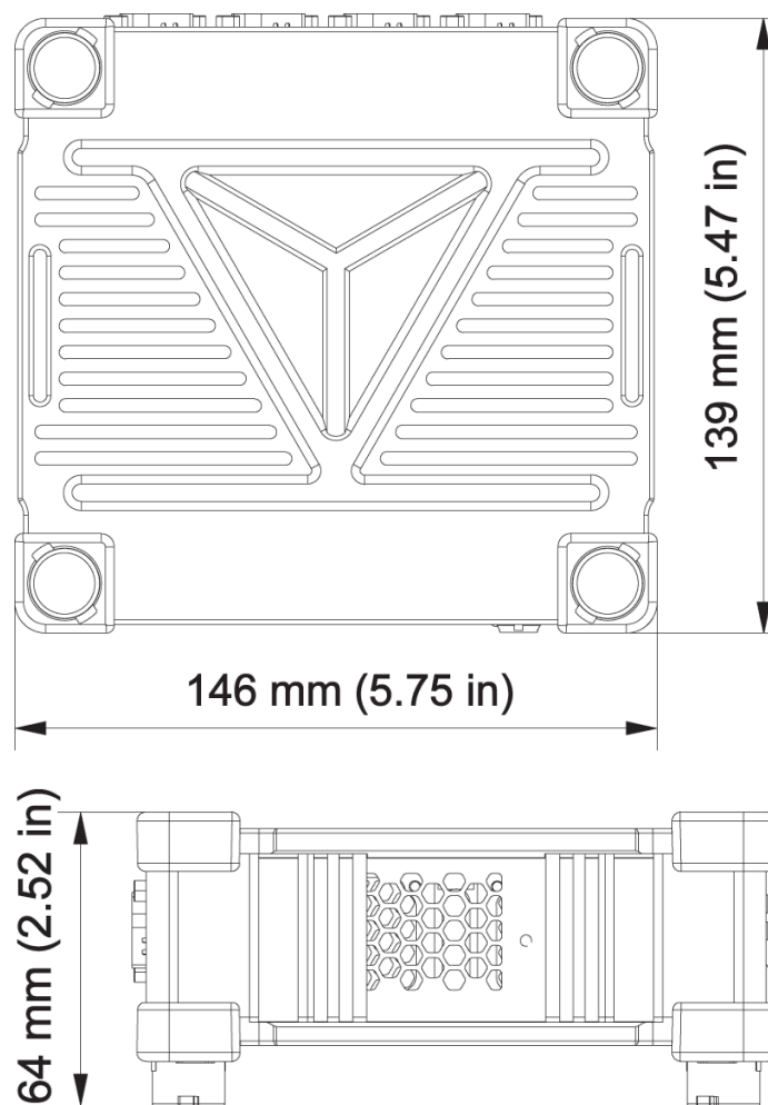
Dimensions: SIRIUSm
