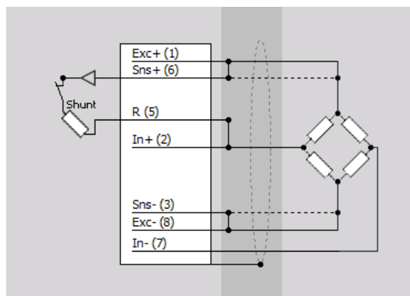
Full bridge
