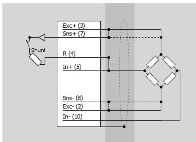
Full bridge
