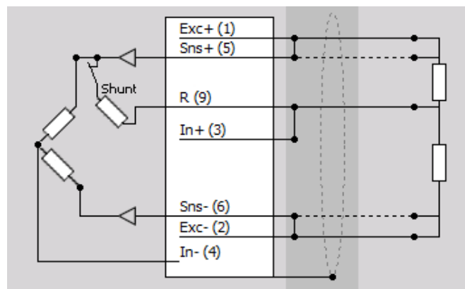
Half bridge
