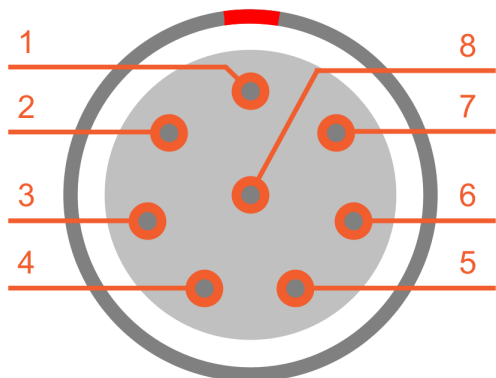
STGM-L2B8f connector: pin-out (LEMO female)
