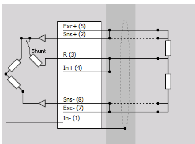
Half bridge
