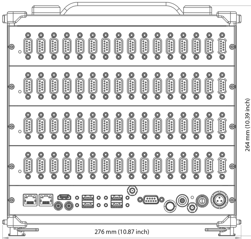
Dimensions: SIRIUS-R4
