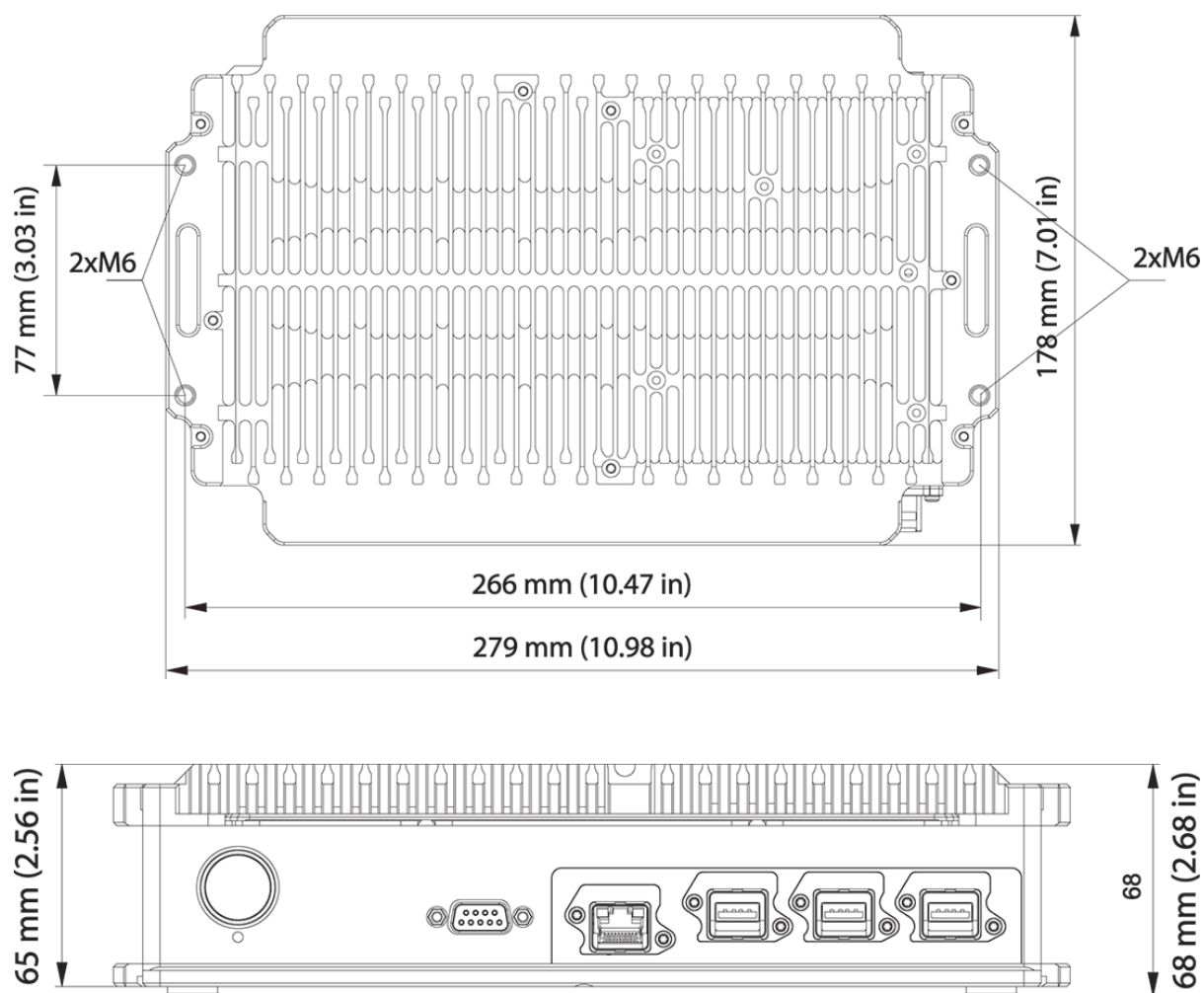
Dimensions: SBOXwe
