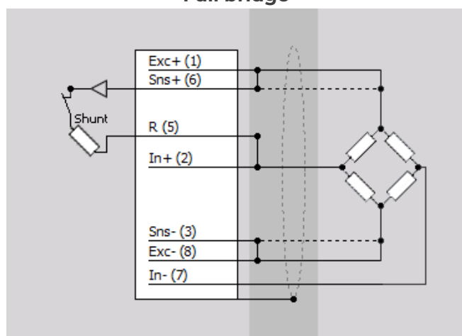
Full bridge
