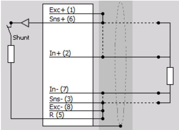
Quarter CC
