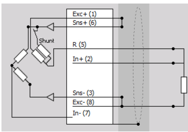
Quarter 3-wire
