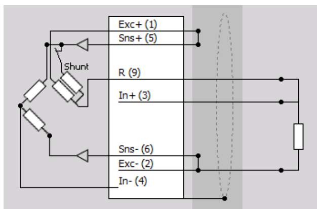
Quarter bridge – 3 wire
