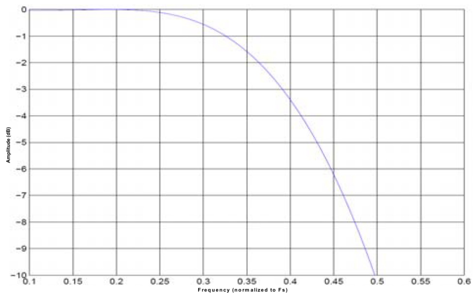
Sample rate 102.4 kHz to 204.8 kHz transition band detail
