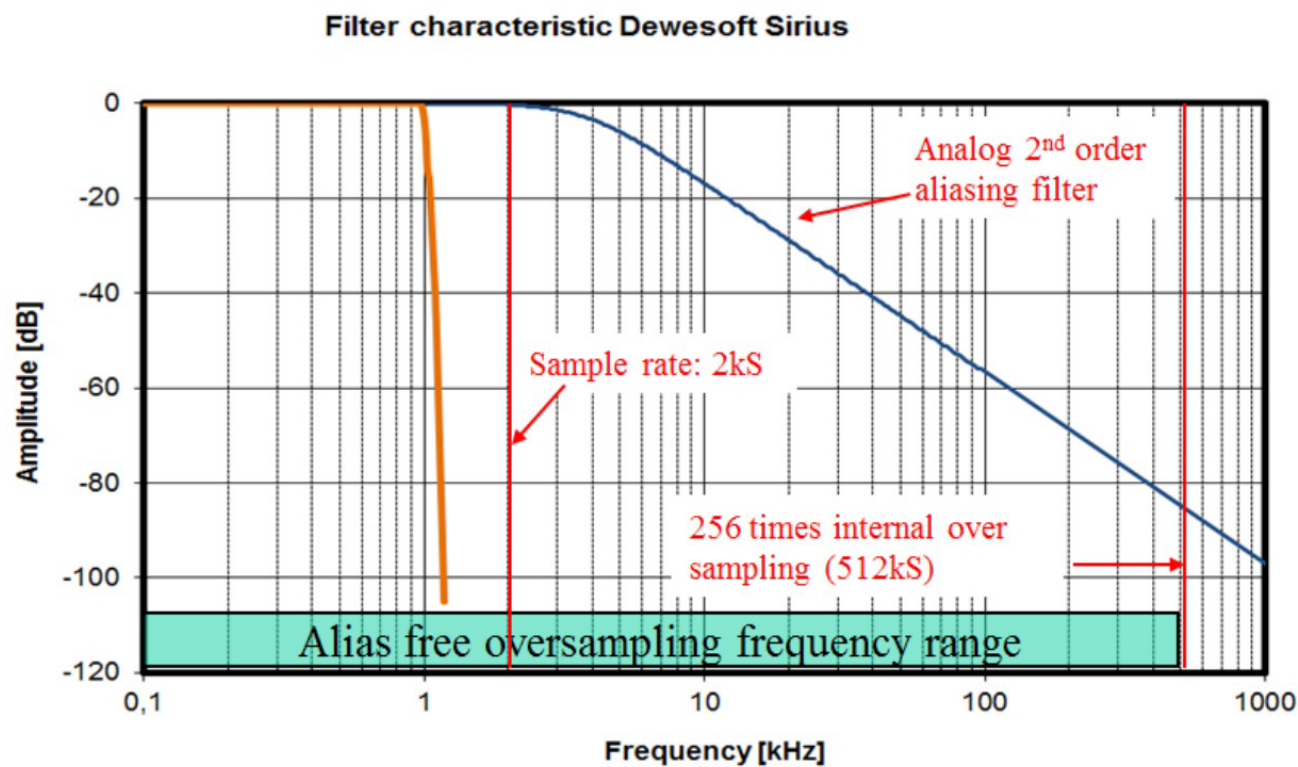
SIRIUS® Anti-Aliasing Filter
