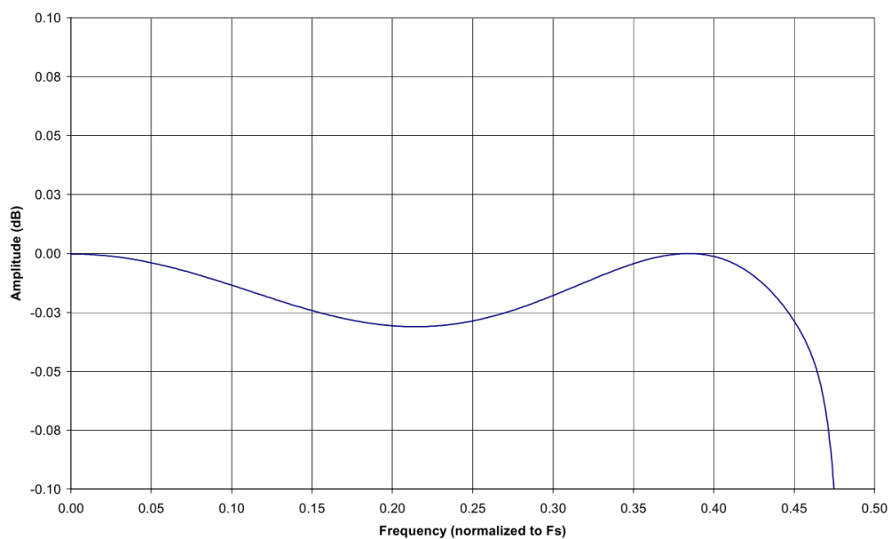
Sample rate 100 Hz to 51.2 kHz Passband ripple
