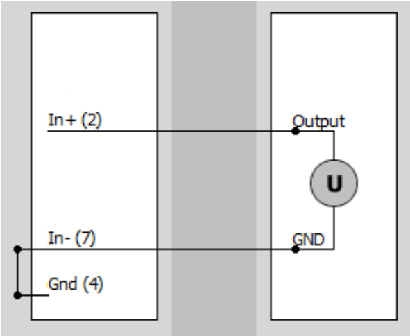
Single ended Input type, Internal electronic switch
