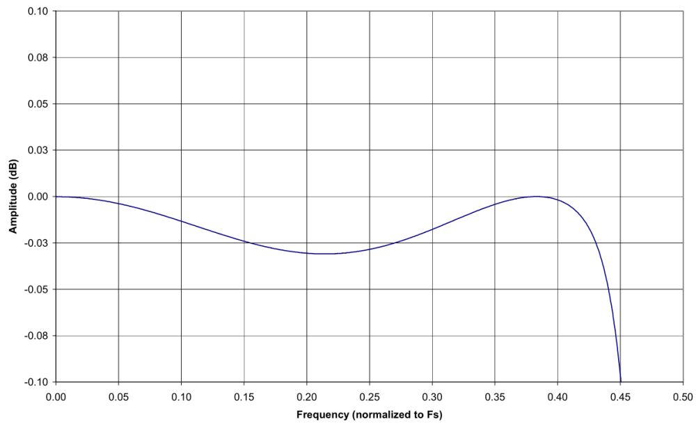
Sample rate 51.2 kHz to 102.4 kHz Passband ripple
