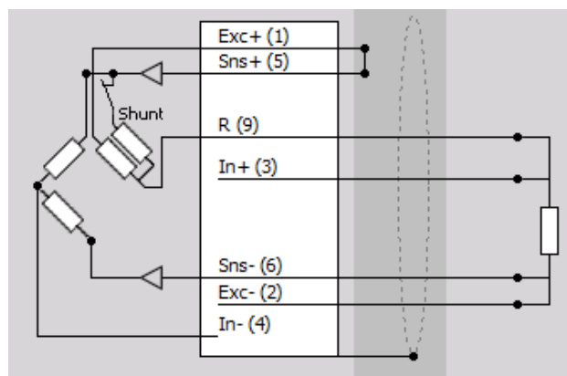
Quarter Bridge – 4 wire
