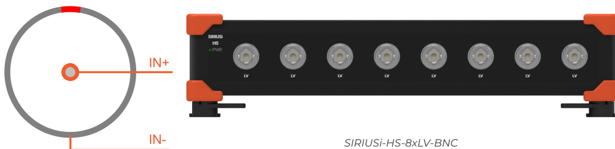
HS-LV-BNC connector: pin-out (BNC)
