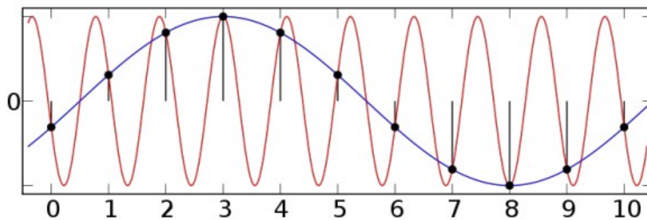
Aliasing effect
