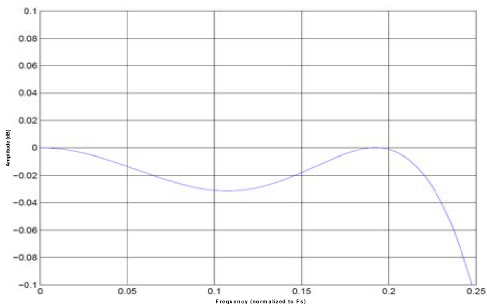
Sample rate 102.4 kHz to 204.8 kHz Passband ripple
