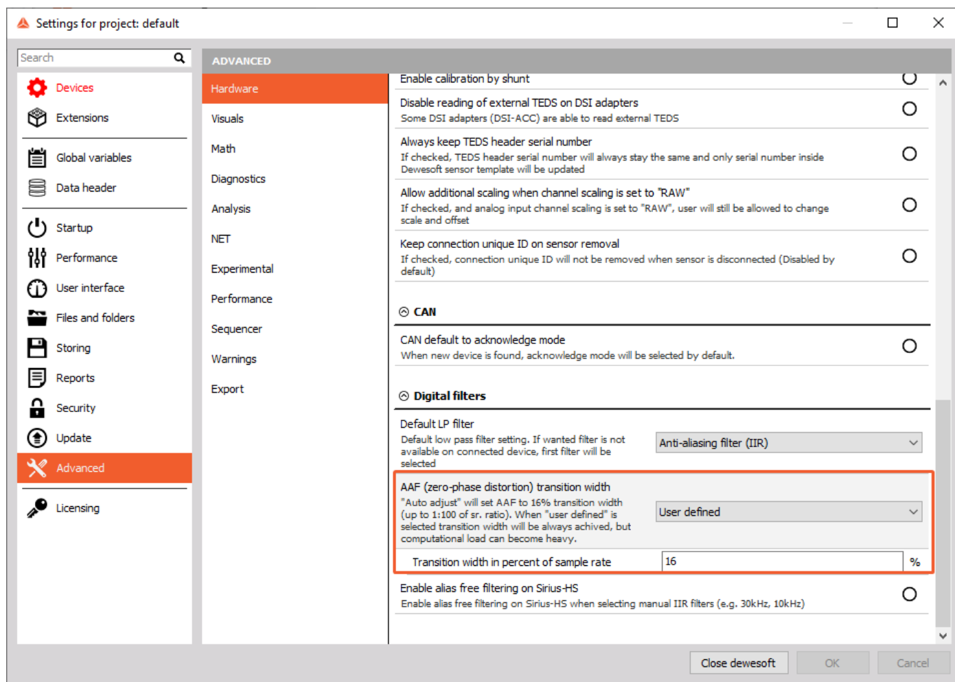
Digital filters, AAF (zero-phase distortion) transition width
