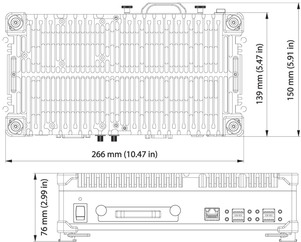
Dimensions: SBOXfe
