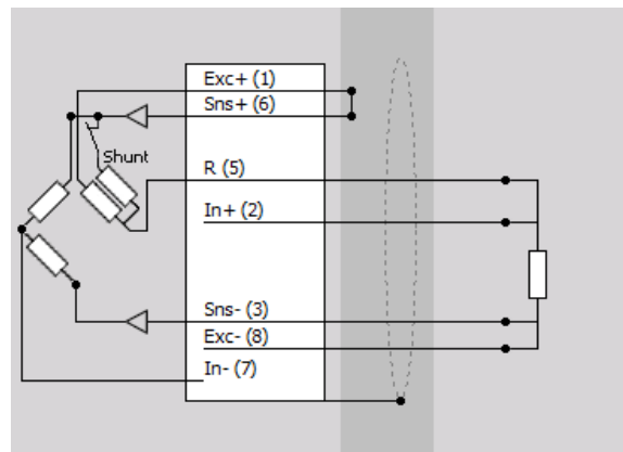
Quarter Bridge – 4 wire
