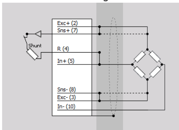
Full bridge
