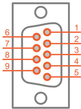
CAN connector: pinout (DSUB-9 male)
