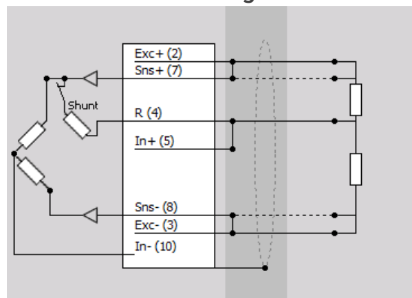
Half bridge
