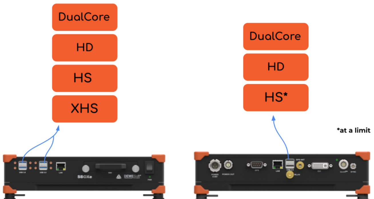
SBOXe Front side (left) and Rear side (right)
