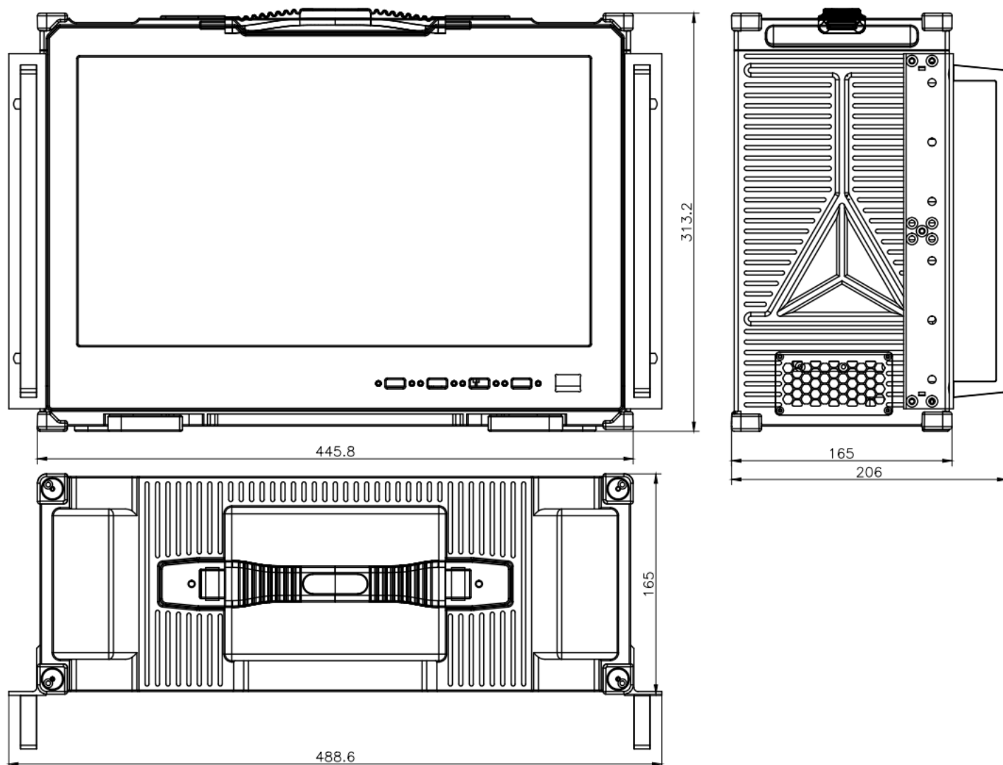
Dimensions: SIRIUS-R8D
