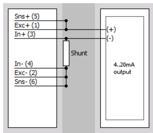
Current - External loop powered shunt
