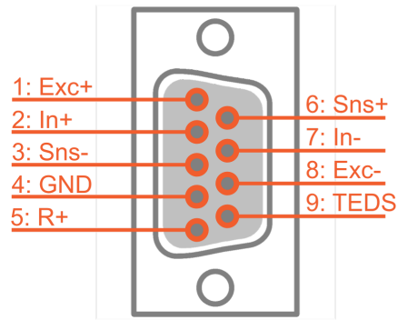
STG connector: pin-out (DSUB-9 female)
