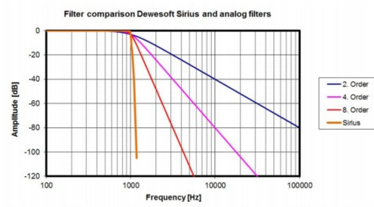
Filter order
