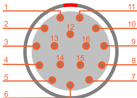
MULTI-L2B16f connector: pin-out
