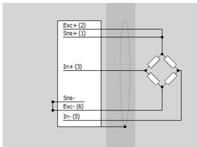
Full bridge
