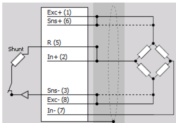
Sns- to In+
