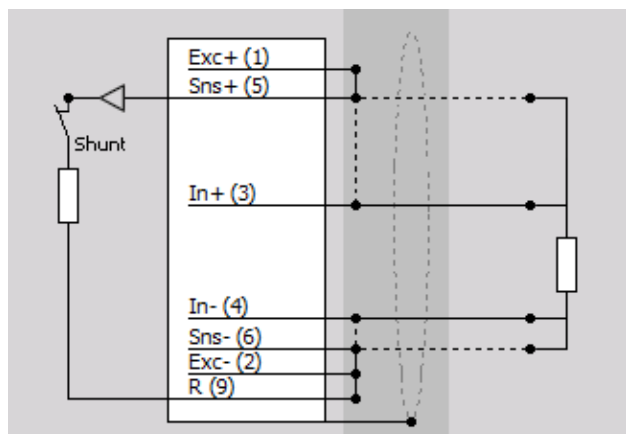
Quarter Bridge – Constant Current
