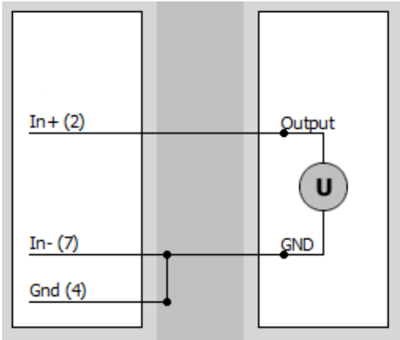
Single ended Input type, External connection required
