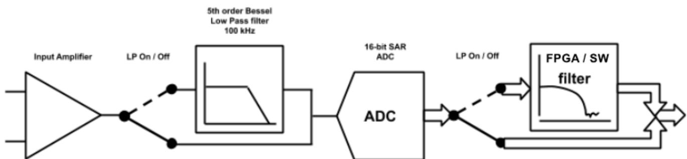
Filtering components in SIRIUS® HS modules
