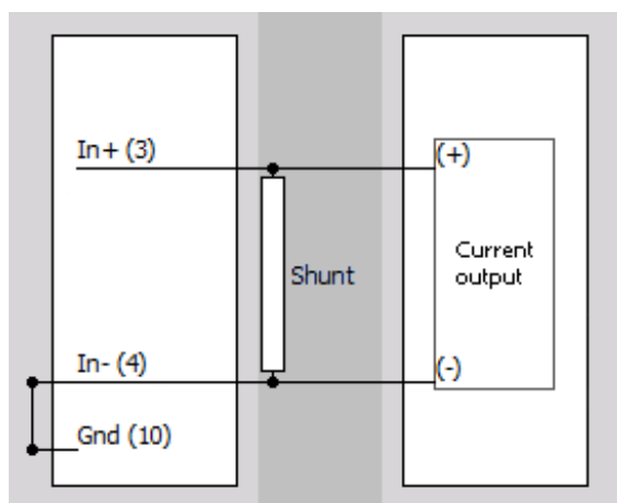
Current - External direct shunt
