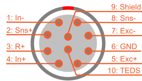
HD-STGS-L1B10f connector: pin-out (10-pin LEMO female)
