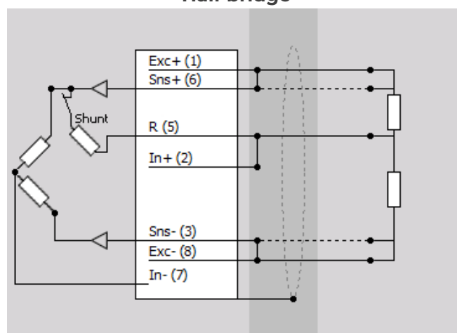
Half bridge
