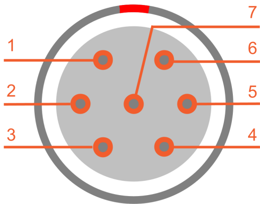
STG-L0B7f connector: pin-out (7-pin LEMO female)
