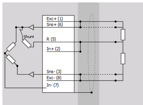
Half bridge
