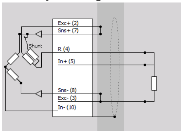
Quarter bridge – 3 wire
