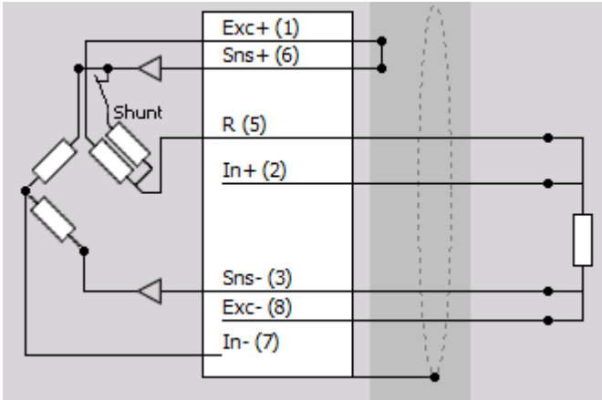
Quarter 4-wire
