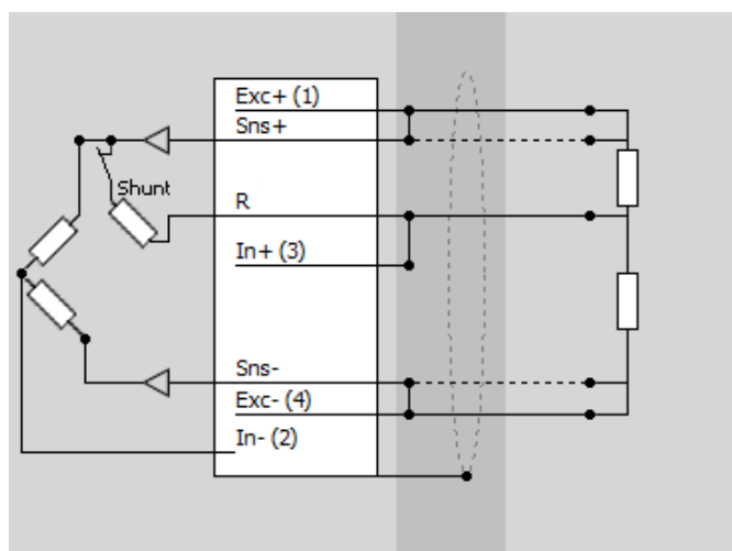
Half bridge
