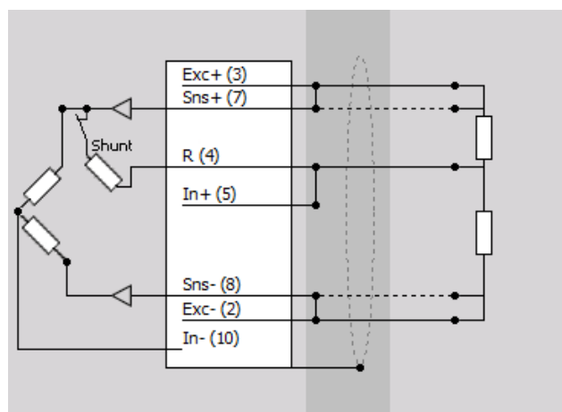
Half bridge
